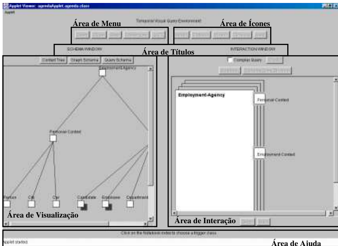
Figura 3.11 – Layout do Applet TVQE
