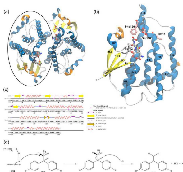
Figure 1. Cartoon representation of the X-ray structure of AgGSTE2 (PDB ID 2IMI). (a) Homodimer; (b) active site in one monomer. Secondary-structure elements are labeled according to Wang et al. ; 17 (c) secondary structure assignment for amino acid sequence from the Protein Databank ( www.rcsb.org ). Only the monomer sequence is represented in Panel C. Residues Ser12 and Glu116 correspond to residues Ser15 and Glu120 respectively in AgGSTE5; (d) schematic representation of the catalysis of DDT by AgGST.
