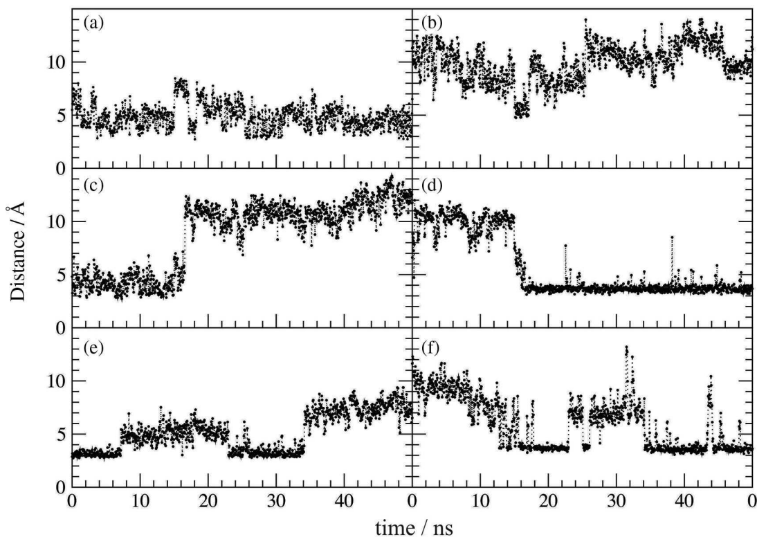
Figure 8. Time-dependent distances between Ser12-GSH (a, c, e) and Glu116-GSH (b, d, f) for (a, b) AgGSTE2, (c, d) AgGSTE2-I114T/F120L, and AgGSTE5 (e, f). Distances were calculated between the center of mass of the hydroxyl group of Ser12 or carboxylate group of Glu116 and the center of mass of the thiol group of GSH.
