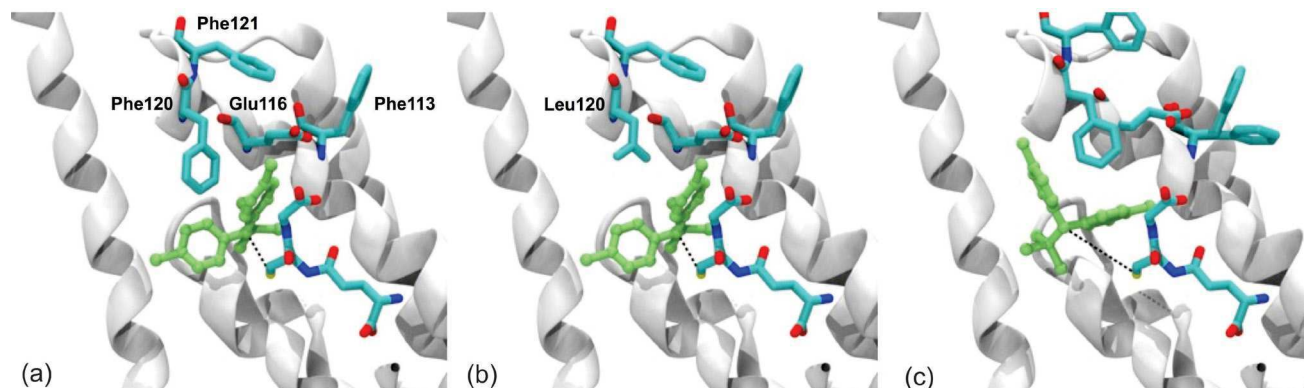
Figure 2. Predicted binding conformation of DDT to AgGSTE2 variants. (a,b) Atomic coordinates from X-ray structure 2IMI solved at 1.4 Å resolution; (c) atomic coordinates from X-ray structure 4GSN solved at 2.4 Å resolution. 1,17 AgGSTE2-I114T/F120L was built by replacement of side chain atoms in mutated residues. DDT is shown in green ball-and-stick. Residues are represented in stick with carbon atoms in cyan, nitrogen in blue, oxygen in red, sulfur in yellow.
