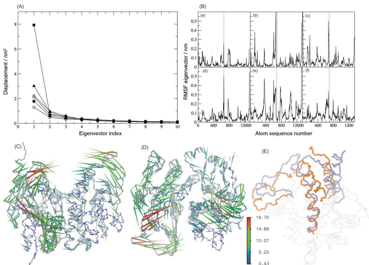
Figure 7. Principal component analysis of MD trajectories. (A) Eigenvalue amplitude for systems AgGSTE2 (circle), AgGSTE2-I114T/F120L (square) AgGSTE5 (triangle). Apoprotein and holoenzyme are represented by open and closed symbols, respectively. (B) Representation of Ca atomic displacement along the first eigenvector for apoenzymes (a) AgGSTE2; (b) AgGSTE2-I114T/F120L; (c) AgGSTE5, and holoenzymes (d) AgGSTE2; (e) AgGSTE2-I114T/F120L; (f) AgGSTE5. (C,D) Porcupine plots representing the highest amplitude motions along the first eigenvector. (E) Superposition of C \alpha atomic coordinates corresponding to the maximum and minimum projections of the first eigenvector for AgGSTE2-I114T/F120L-GSH.
