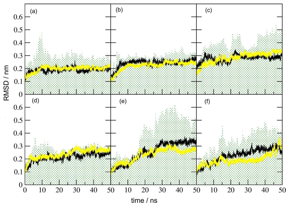
Figure 4. Root-mean-square deviation of C \alpha atoms from X-ray structure for the apoenzymes (a) AgGSTE2; (b) AgGSTE2-I114T/F120L; (c) AgGSTE5; and the holoenzymes (d) AgGSTE2; (e) AgGSTE2-I114T/F120L; (f) AgGSTE5. Root-mean-square deviations were calculated for C \alpha atoms in subunit A (black), subunit B (yellow) and in the full dimer (green dots). The X-ray structures 2IL3 and 2IMI were used as positional reference for the apo and holoenzymes, respectively.
