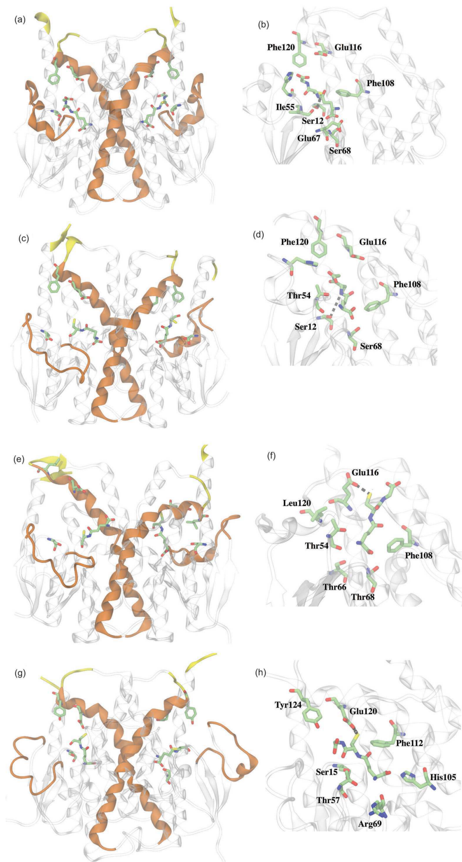
Figure 6. Conformational changes involving helices H2, H4 and the C-terminal region of AgGSTE variants during MD simulations. The structural rearrangement places Glu116 within hydrogen bond distance of the thiol group of GSH. (a,b) X-ray structure (2IMI); (c,d) final conformations from MD simulations of AgGSTE2; (e,f) AgGSTE2-I114T/F120L; (g,h) AgGSTE5.
