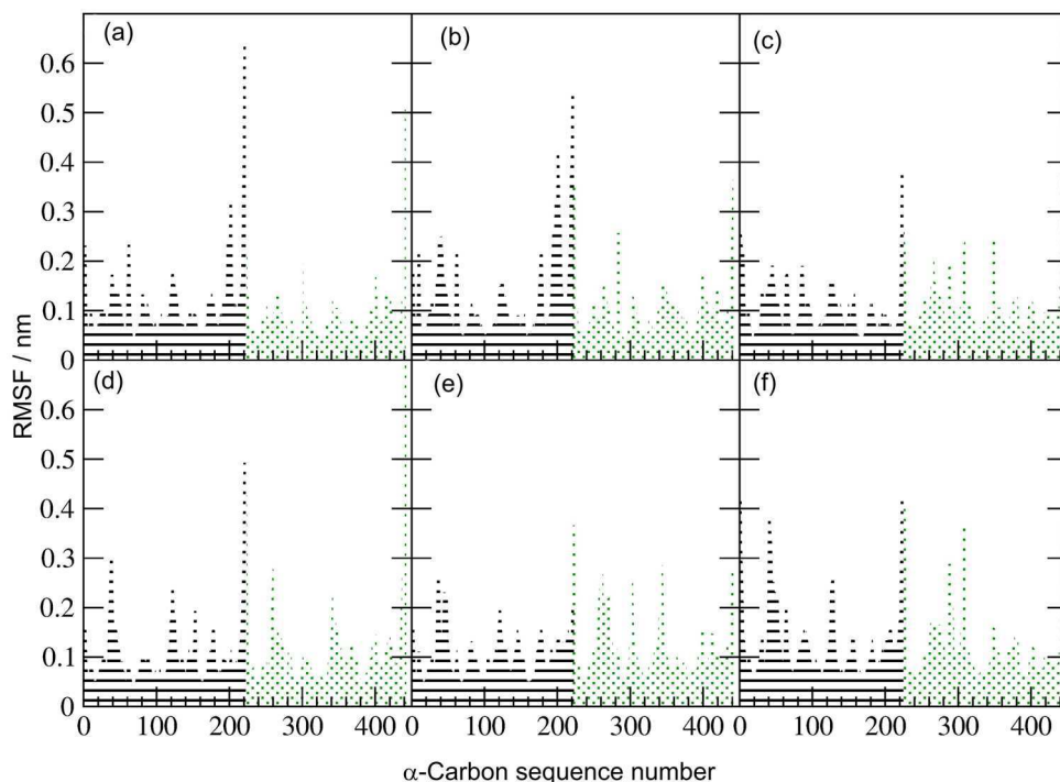
Figure 5. Root-mean-square fluctuation of C \alpha atoms for the apoenzymes (a) AgGSTE2; (b) AgGSTE2-I114T/F120L; (c) AgGSTE5; and the holoenzymes (d) AgGSTE2; (e) AgGSTE2-I114T/F120L; (f) AgGSTE5. Rotational and translational fitting of pairs of structures was applied using C \alpha atoms. RMSF values were calculated for the final 25 ns of simulation.
