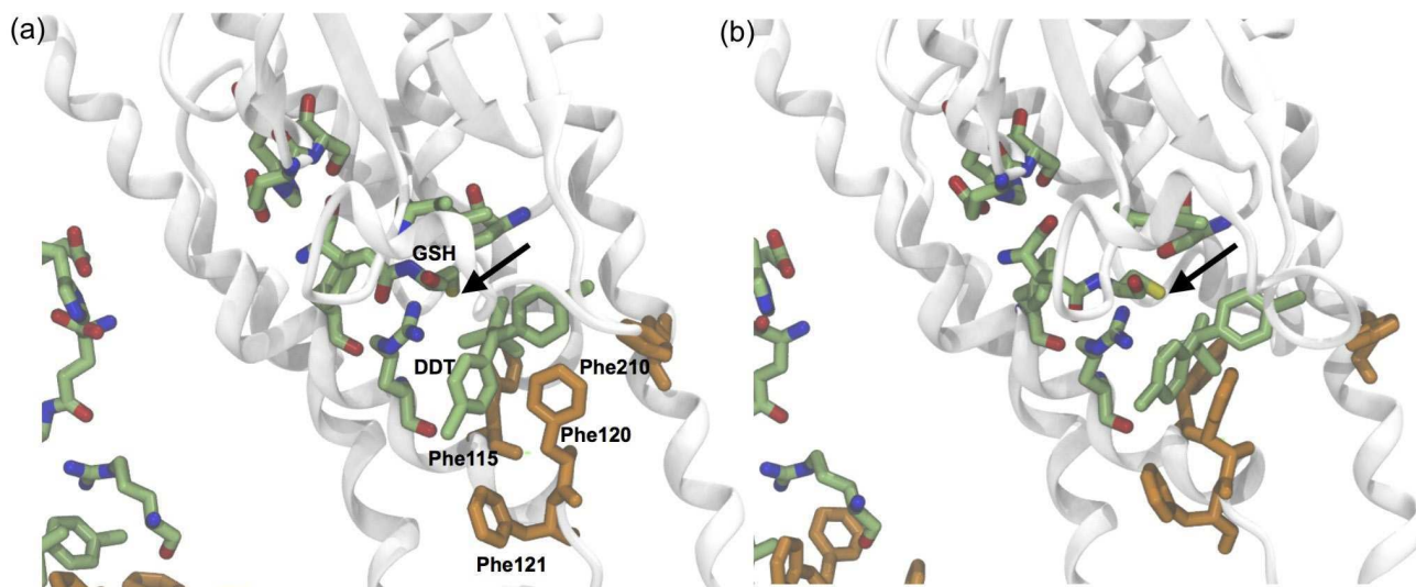
Figure 3. (a) Initial; (b) final conformation of AgGSTE2 bound to DDT. Residues are represented in stick with carbon atoms in green, nitrogen in blue, oxygen in red, sulfur in yellow. Phenylalanine residues surrounding DDT are shown in orange. Black arrows indicate the thiolate anion from GSH. Hydrogen atoms are not shown for clarity.
